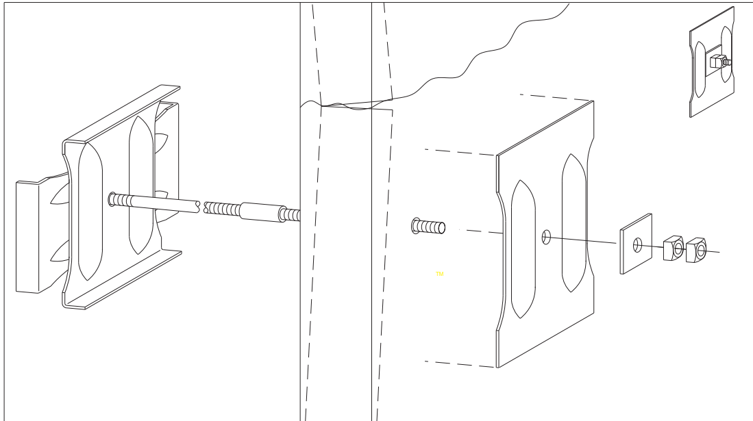
TYPICAL INSTALLATION OF DURA-GRIP WALL ANCHOR KIT
