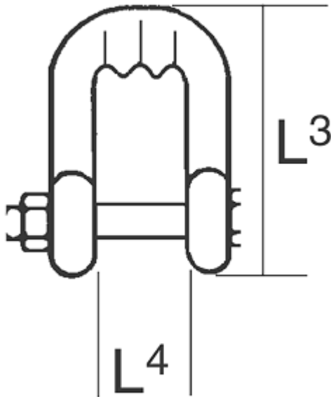
Tripleye Chain Shackle SS 150
