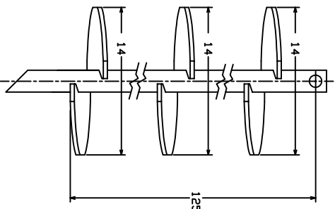
LEAD SECTION C110-0572 (GALV) C114-0216 (UNGALV)
