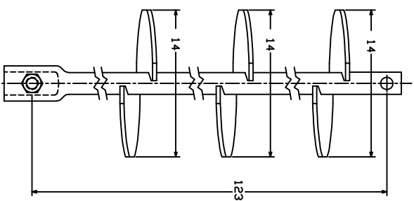
THREE HELIX EXTENSION C110-0586 (GALV) C114-0231 (UNGALV)
