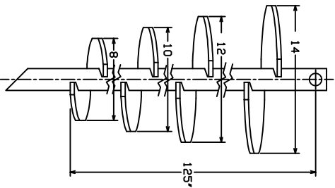
LEAD SECTION C110-0573 (GALV) C114-0217 (UNGALV)
