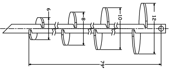
LEAD SECTION C110-0571 (UNGALV)
