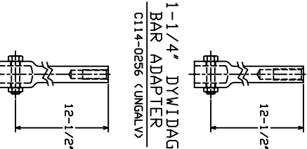
1" DYWIDAG BAR ADAPTER C114-0227 (GALV)
