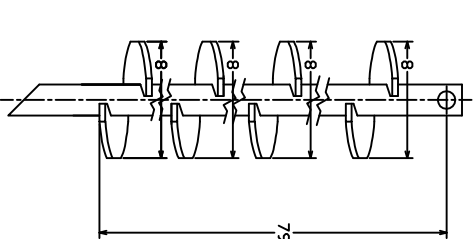
LEAD SECTION C114-0218 (GALV)
