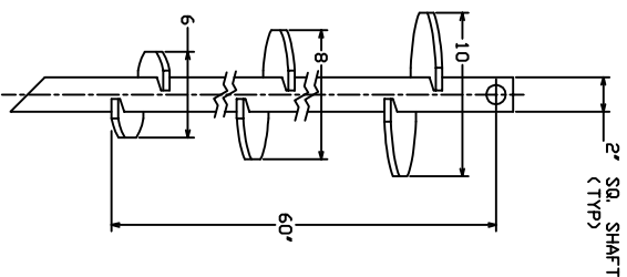
LEAD SECTION C110-0569 (GALV) C114-0214 (UNGALV)
