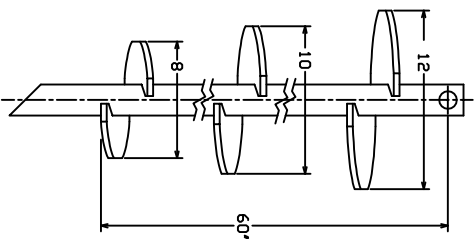
LEAD SECTION C110-0570 (GALV) C114-0215 (UNGALV)
