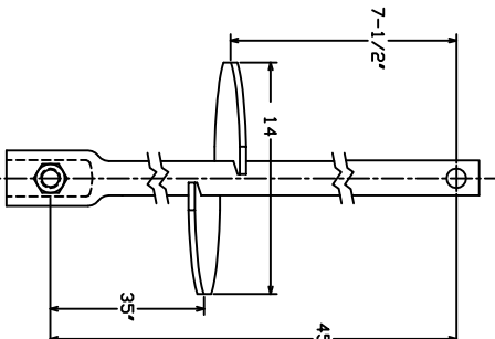
SINGLE HELIX EXTENSION C110-0577 (GALV) C114-0220 (UNGALV)
