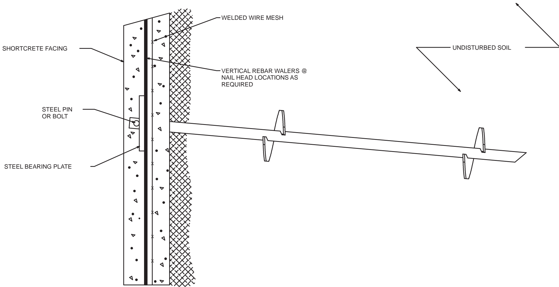
TYPICAL FACING SYSTEM FOR A TEMPORARY SOIL SCREW RETENTION WALL SYSTEM™
