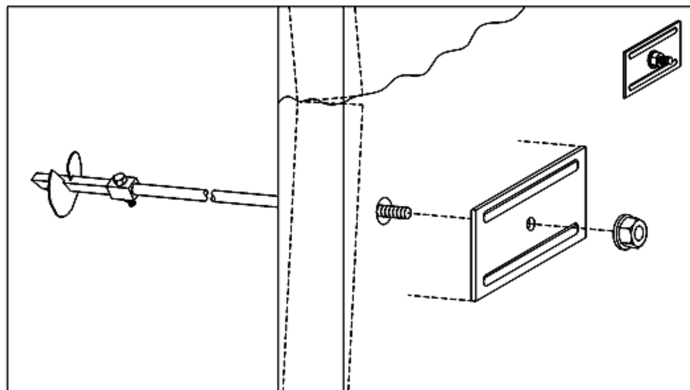
TYPICAL INSTALLATION OF WALL ANCHOR KIT
