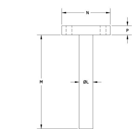
FIGURE 6—T-PIPE FOR STANDARD AND HEAVY-DUTY REMEDIAL REPAIR BRACKETS
