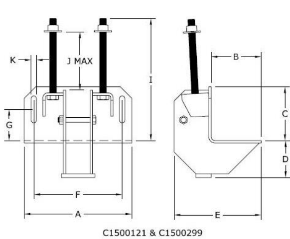
FIGURE 3—STANDARD REMEDIAL REPAIR BRACKETS
