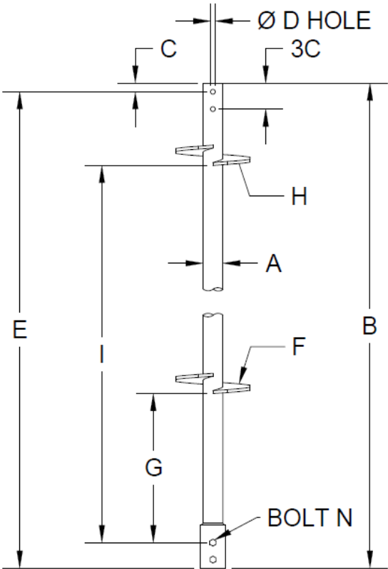
FIGURE 1B—RS2875.276 & RS3500 LEAD SECTIONS
