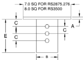
FIGURE 7B—NEW CONSTRUCTION PILE CAP FOR RS2875.276 & RS3500
